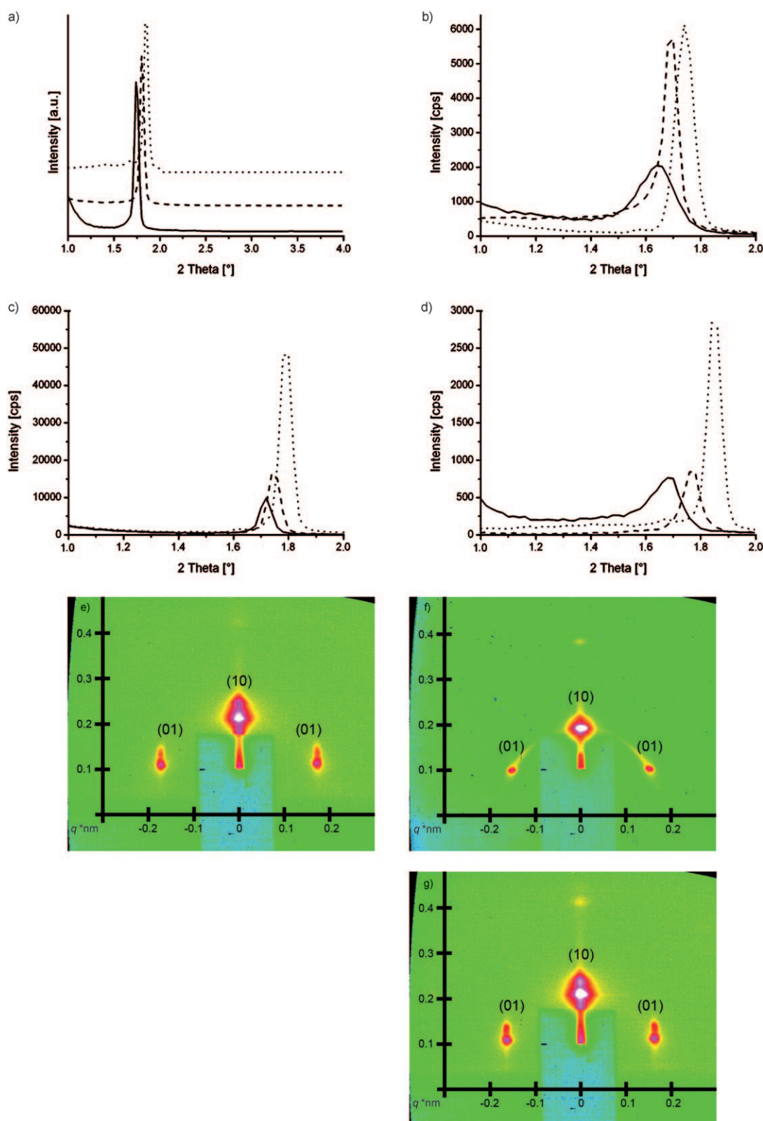
Figure 1. Structural analysis. a–d) 1D X-ray diffractograms of functionalized silica films with varying lengths of alkyl-chains (a; methyl (—), ethyl (---), propyl (·····); functionalization density 10 mol %, normalized to the reflection with maximum intensity), with varying amounts of cyanopropyl functionalization (b; 5.0 (—), 10 (---), and 20 mol % (·····)), with varying amounts of phenyl-functionalization (c; 5.0 (—), 10 (---), and 20 mol % (·····)), and with varying amounts of propyl functionalization (d; 2.5 (—), 5 (---), and 10 mol % (·····)). e–g) GISAXS patterns of 10 mol % propyl-functionalized (e), 20 mol % cyanopropyl-functionalized (f), and 20 mol % phenyl-functionalized (g) silica films. The double peaks in e) and g) arise at very low incident angles when the distorted-wave Born approximation becomes important for highly reflective surfaces. [29] At very low angles the incoming beam can be reflected from the substrate and then scattered by the top film, and this leads to the observed shift of Bragg-like peaks to higher angles. The lower the incoming angle the larger the distance between the two reflections.
